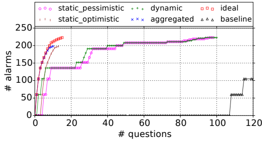
Fig. 10. Number of questions asked and number of false alarms eliminated by URSA with different Heuristic instantiations.
